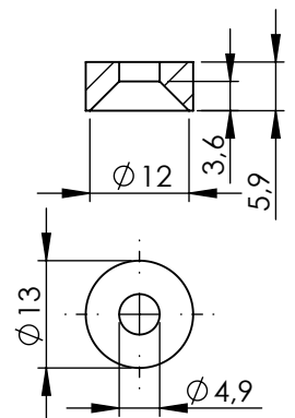
Schraubenbuchse screw bush
